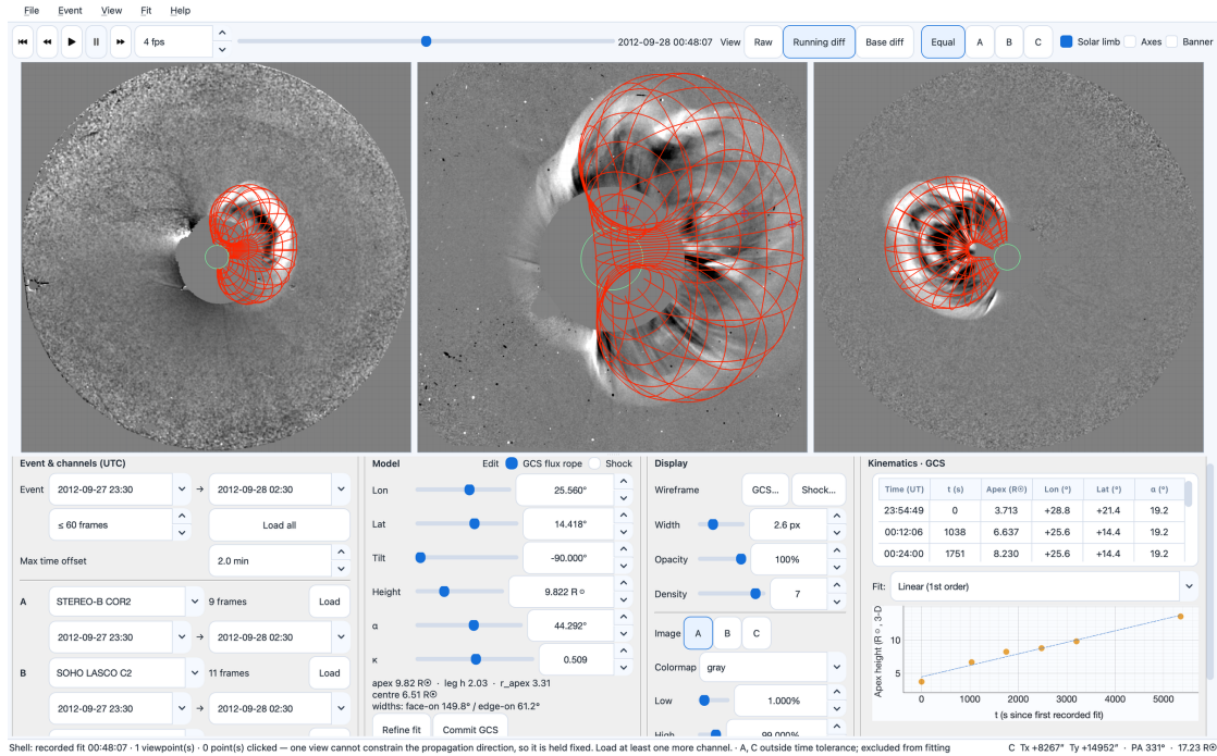
Figure 21.2 A GCS fit with three recorded times; the Kinematics card (right) lists the recorded fits beside their height–time graph and linear fit.
