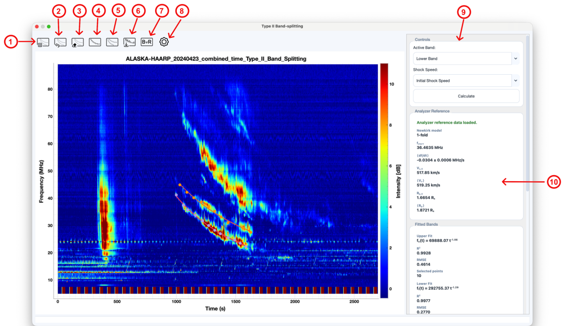
Figure 9.1 The Type II Band-splitting window with its tools and panels numbered.
