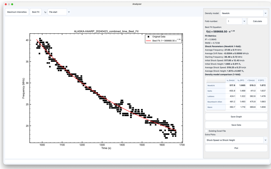
Figure 8.6 The Burst Analyzer window with the best fit, shock parameters and density-model comparison.
