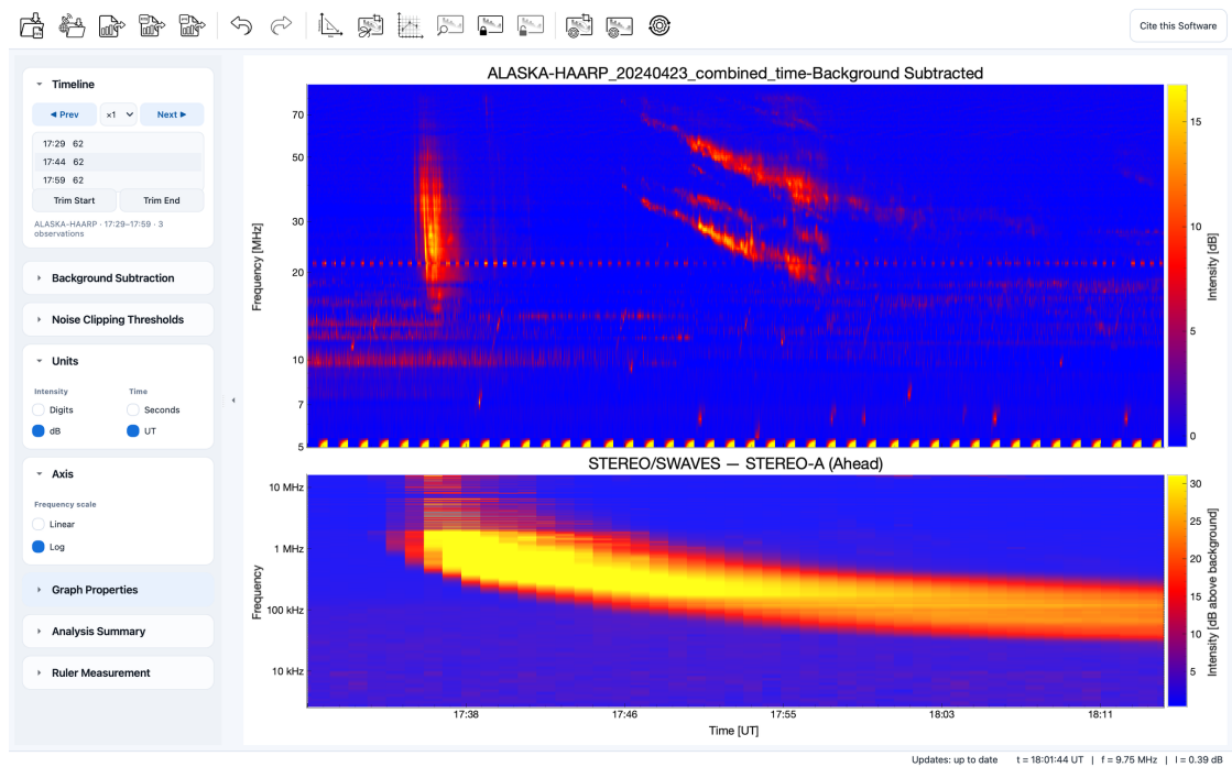
Figure 13.3 CALLISTO and STEREO/SWAVES spectra in the split view.
