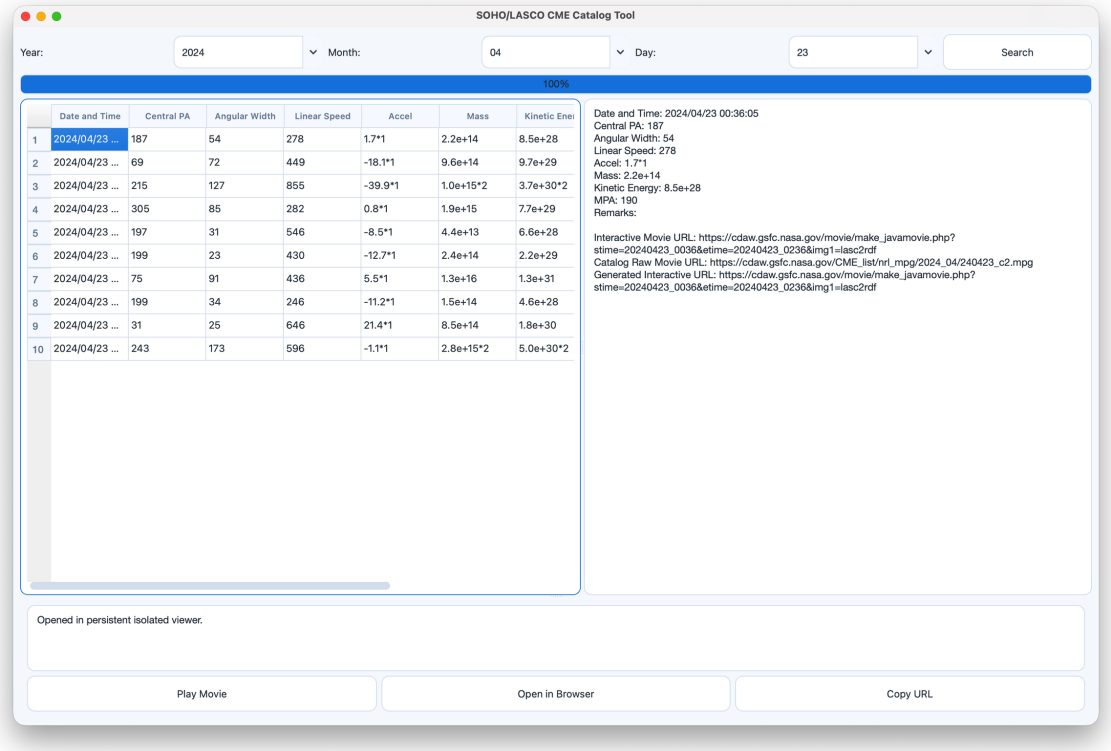
Figure 14.6 The SOHO/LASCO CME Catalog Tool.
