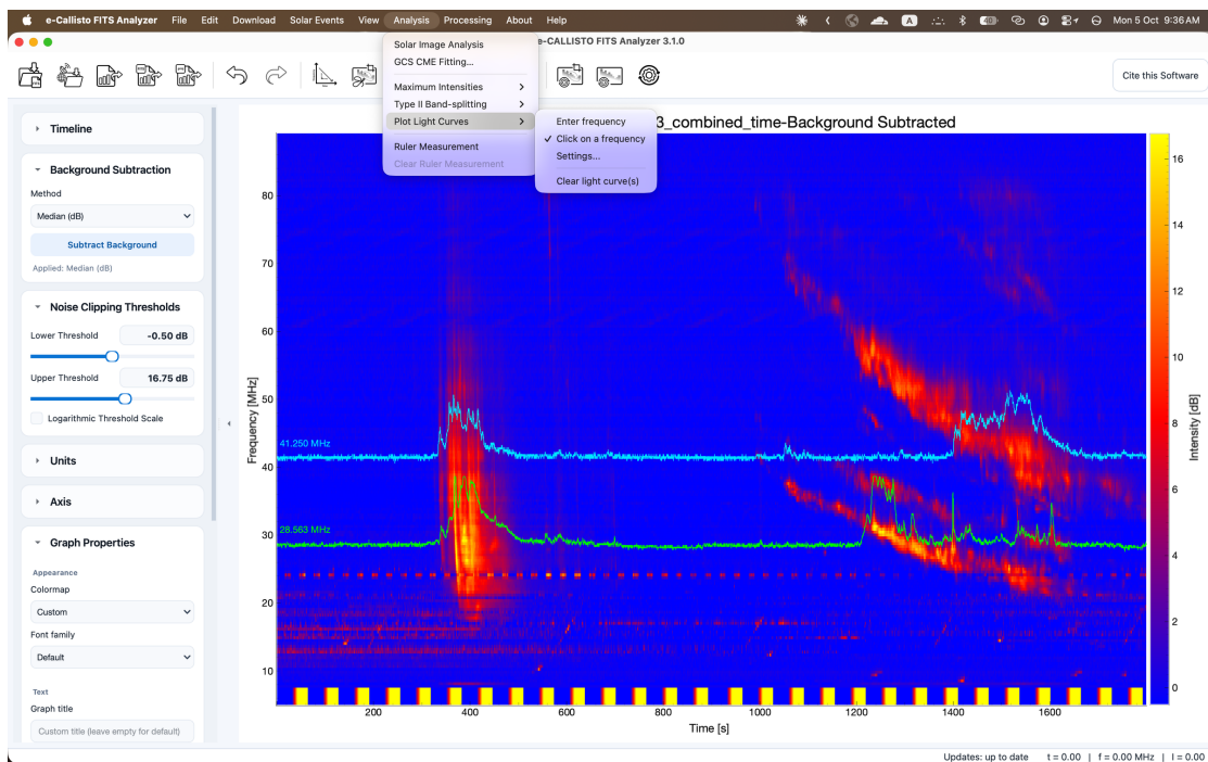
Figure 7.4 Light curves at two frequencies overlaid on a dynamic spectrum, with the Analysis → Plot Light Curves submenu open.
