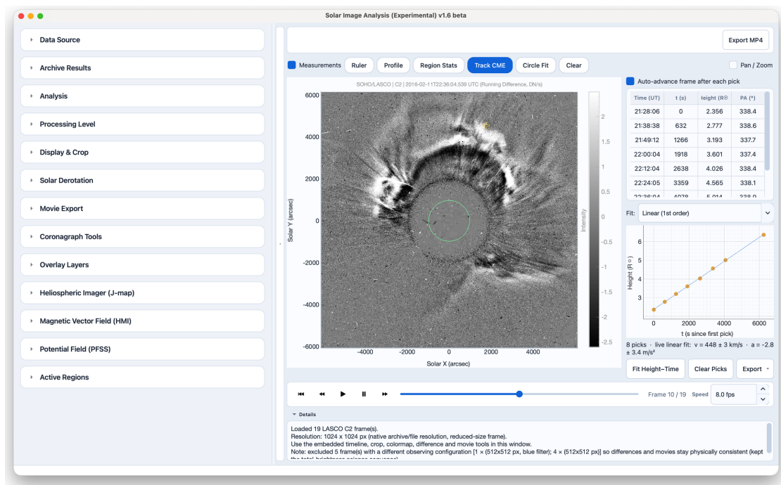
Figure 18.1 CME tracking with the height–time graph in the tracking panel.
