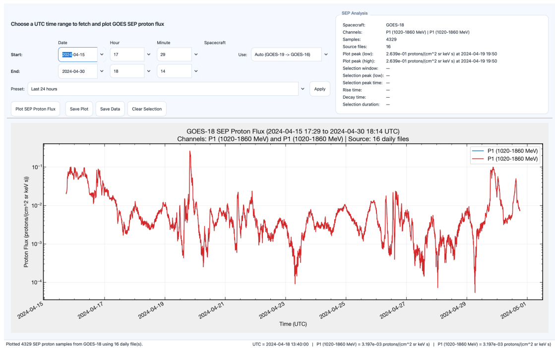
Figure 14.3 The GOES SEP Proton Flux Plotter.
