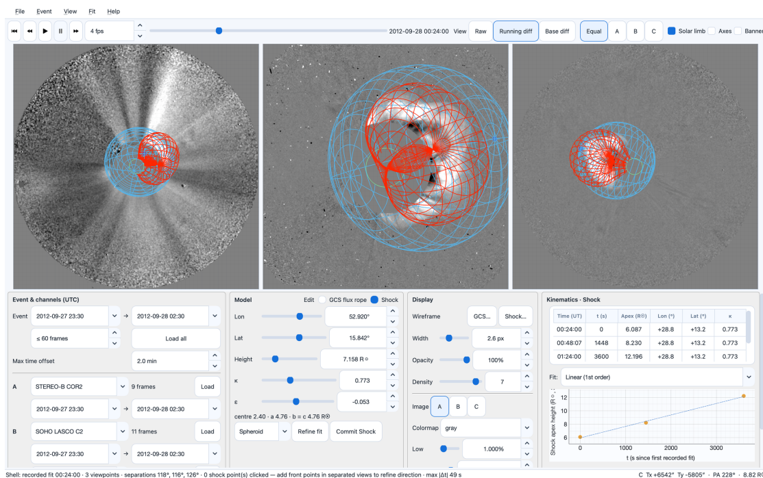
Figure 21.3 Shock and flux-rope models in three viewpoints.
