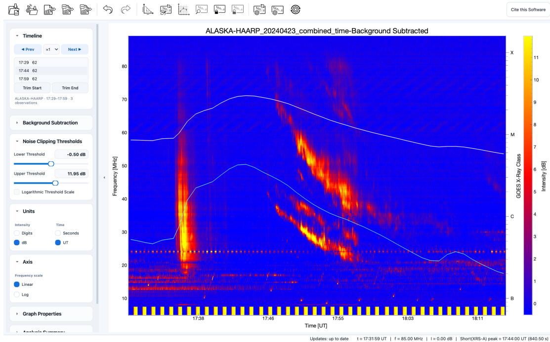
Figure 14.2 GOES X-ray curves overlaid on a dynamic spectrum.
