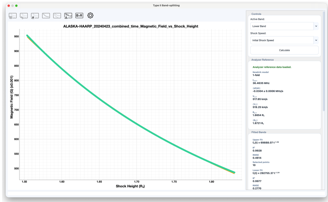
Figure 9.2 Magnetic field versus shock height in the band-splitting window.
