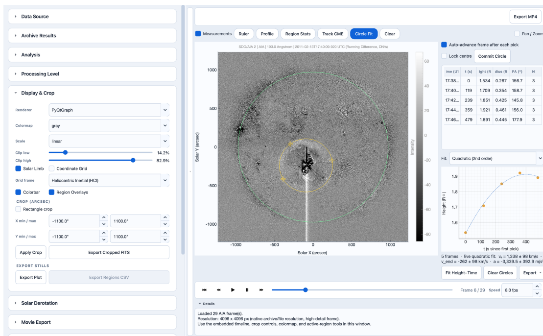
Figure 18.2 Circle fitting of an on-disk CME front.
