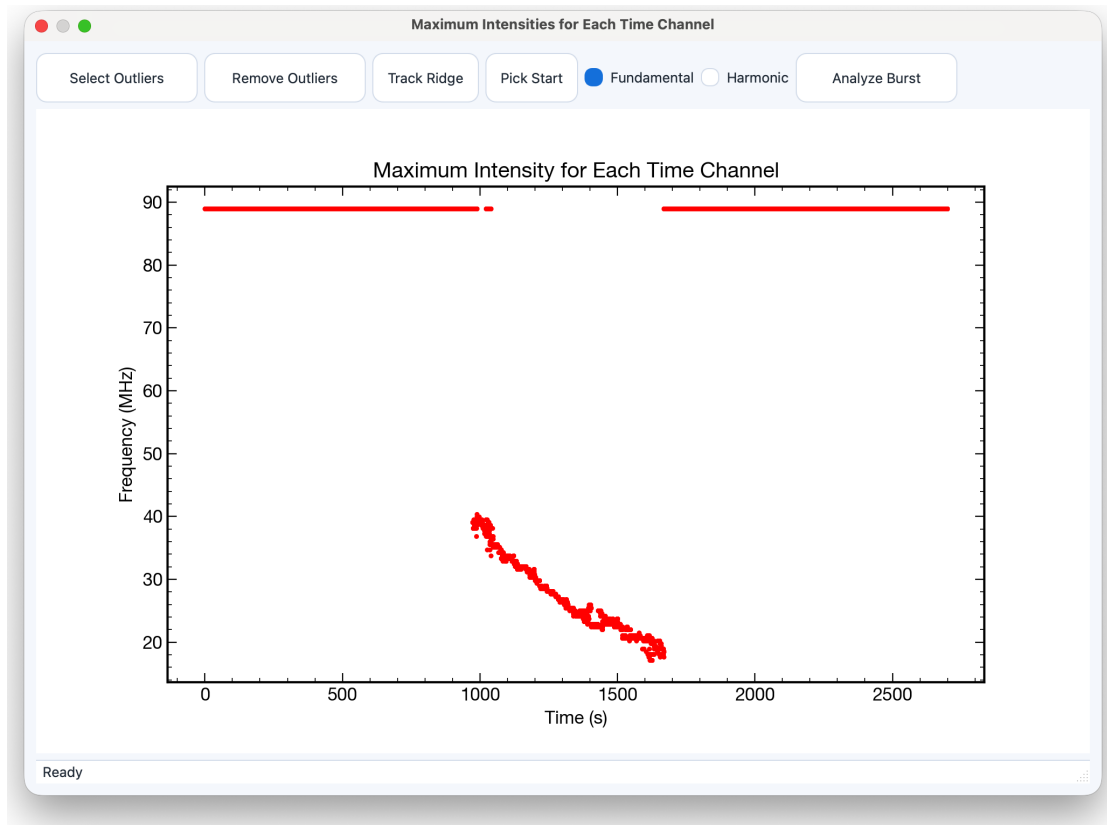
Figure 8.3 The Maximum Intensities window. Without isolation, a persistent RFI channel near 89 MHz produces spurious points.
