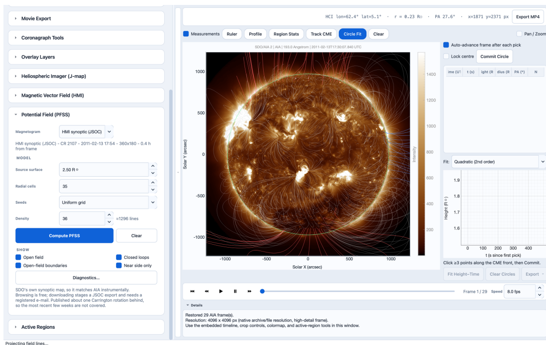
Figure 19.1 PFSS field lines over an AIA image.
