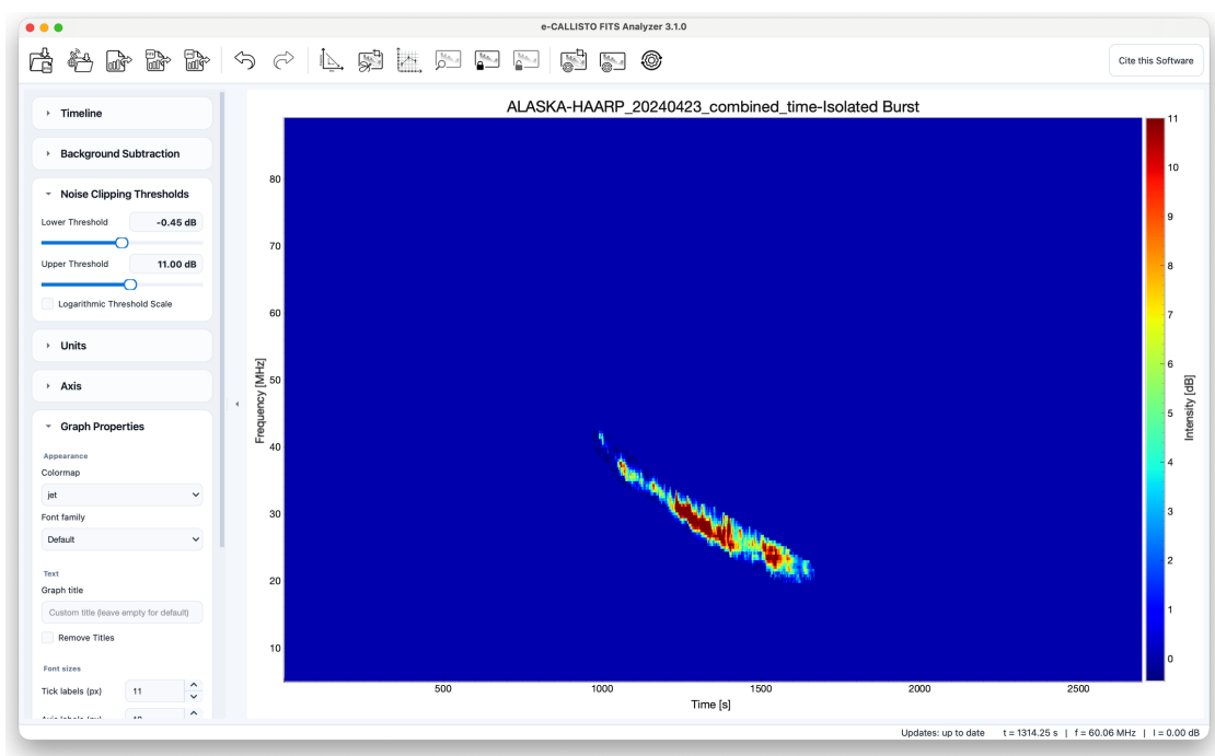
Figure 8.2 An isolated Type II burst lane.
