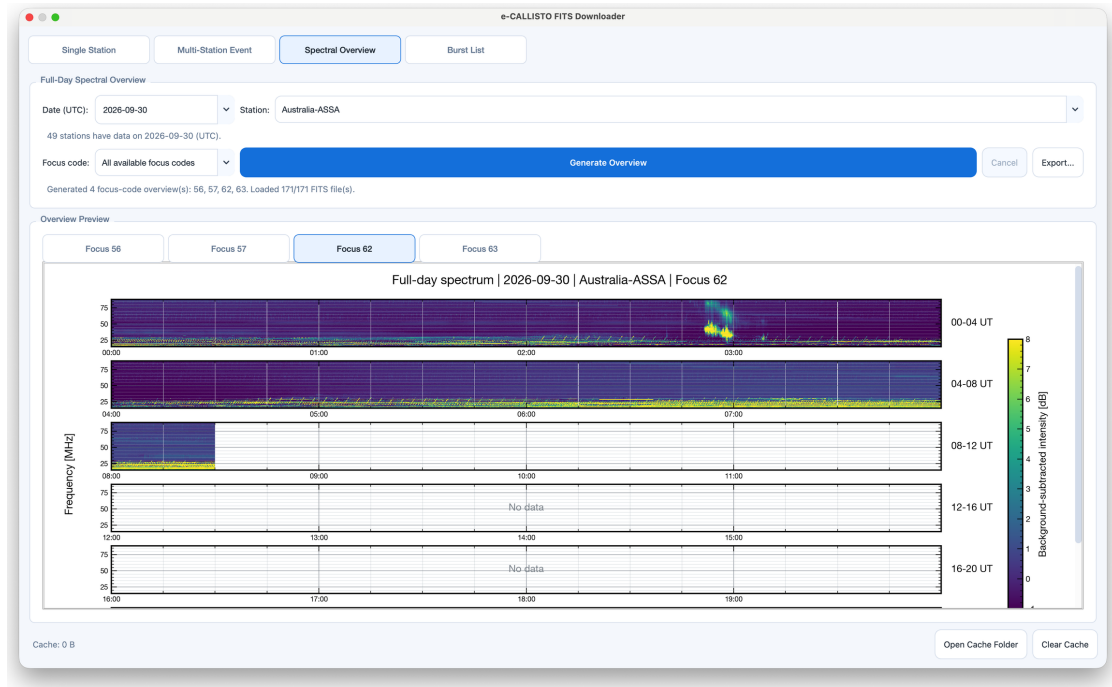
Figure 11.3 The Spectral Overview tab with a full-day overview for one focus code.
