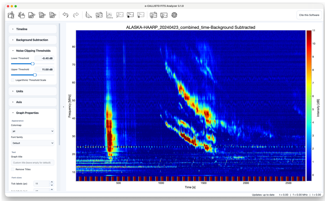
Figure 8.1 A background-subtracted dynamic spectrum containing a Type II burst.
